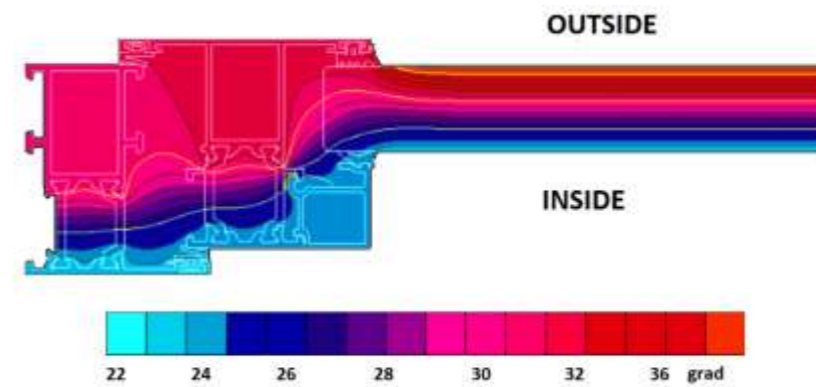
This picture shows the temperature variation in our thermal break profile. Outside HOT , inside COLD !
